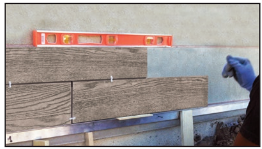
Use a rigid aluminum channel to support and level the first row of tiles during installation.
